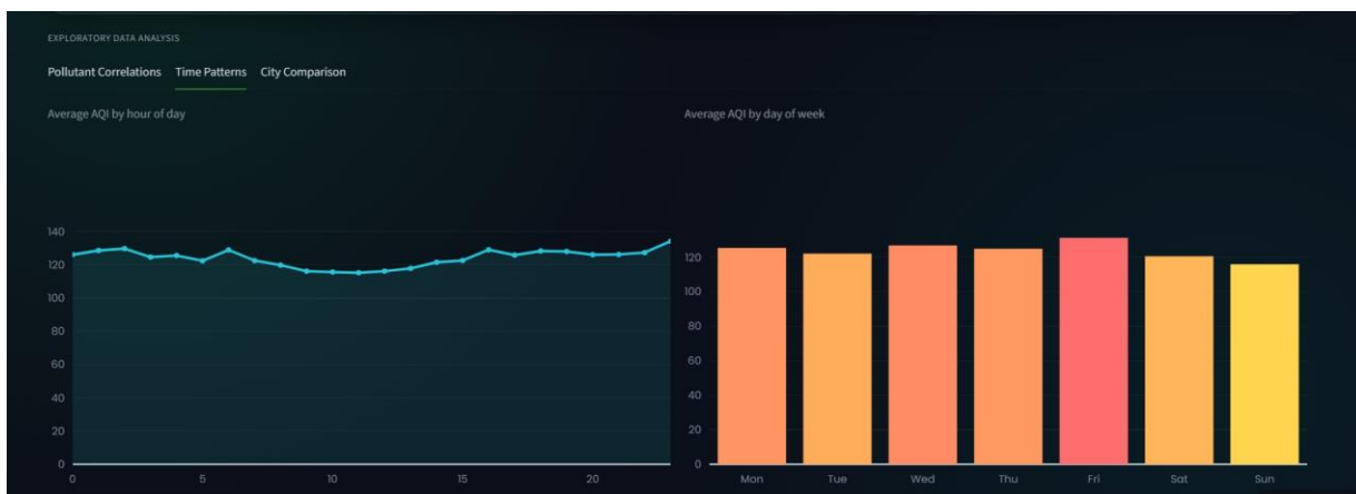
Figure 6: AQI by Hour of Day and Day of Week
